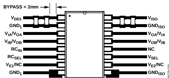
Figure 23. Recommended PCB Layout
