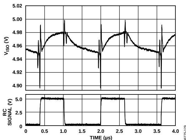
Figure 15. Typical Output Voltage Ripple at 90% Load, V_{ISO} = 5 V
