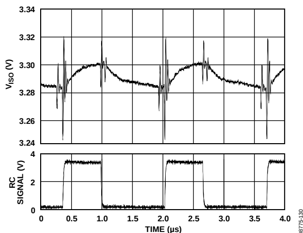
Figure 16. Typical Output Voltage Ripple at 90% Load, V_{ISO} = 3.3 V
