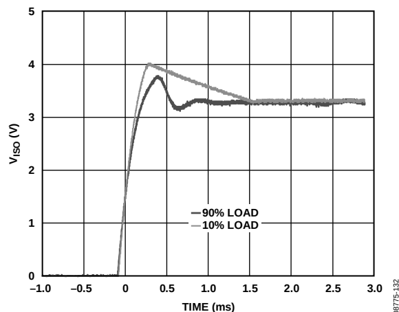
Figure 18. Typical Output Voltage Start-Up Transient at 10% and 90% Load, V_{ISO} = 3.3 V
