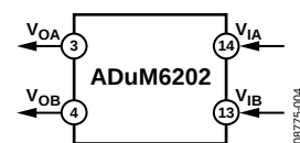
Figure 4. ADuM6202
