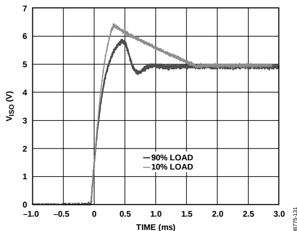
Figure 17. Typical Output Voltage Start-Up Transient at 10% and 90% Load, V_{ISO} = 5 V
