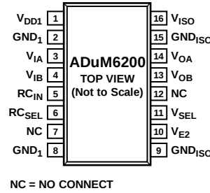
Figure 6. ADuM6200 Pin Configuration
