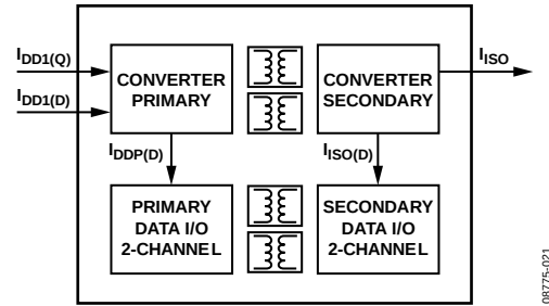
Figure 27. Power Consumption Within the ADuM620x
