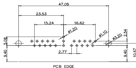
CODE:21W1 MALE/FEMALE
