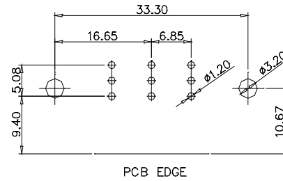
CODE:3W3/3WK3 MALE/FEMALE
