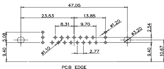
CODE:17W2 MALE/FEMALE
