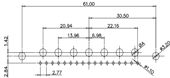
CODE:21W4 MALE/FEMALE
