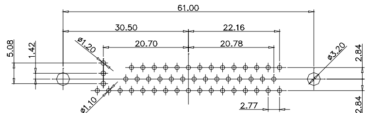
CODE:47W1 FEMALE
