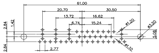
CODE:36W4 MALE
