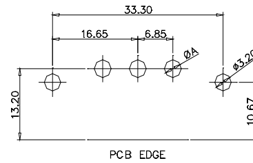
CODE:8W8 MALE
