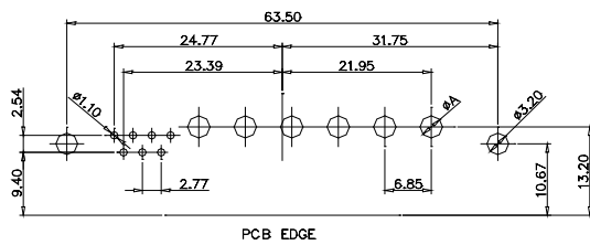
CODE:13W6 FEMALE
