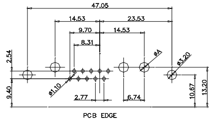
CODE:13W3 FEMALE
