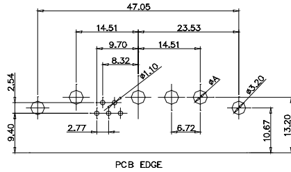
CODE:9W4 FEMALE
