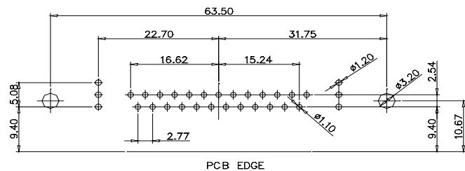
CODE:21W1 MALE/FEMALE
