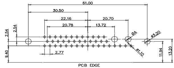
CODE:43W2 MALE
