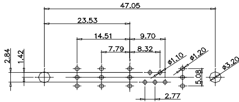
CODE:9W4 MALE
