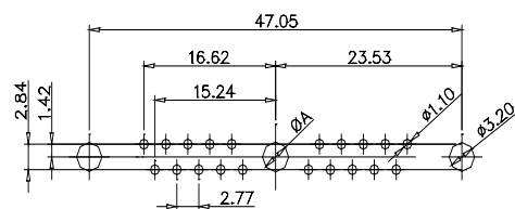
CODE:21W1 MALE/FEMALE
