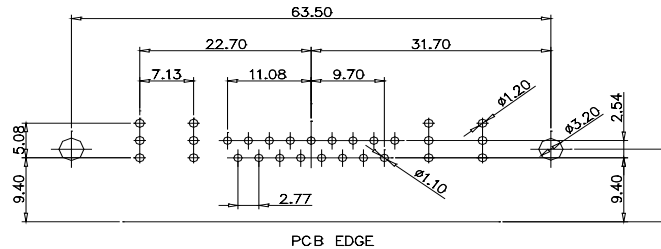
CODE:21W4 MALE/FEMALE
