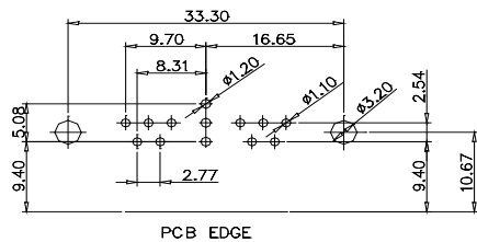
CODE:17W2 MALE/FEMALE
