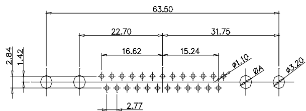
CODE:21W1 MALE/FEMALE
