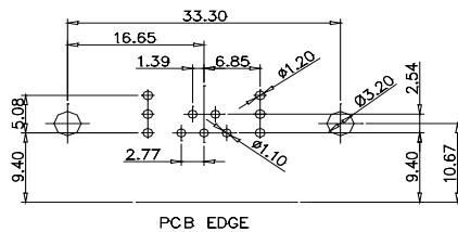
CODE:11W1 MALE/FEMALE
