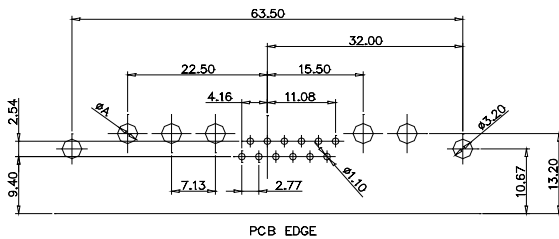
CODE:17W5 FEMALE
