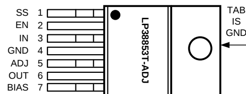
Figure 2. TO-220-7 – Top View See Package Number NDZ0007B
