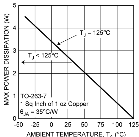
Figure 34. Maximum Power Dissipation vs Ambient Temperature for the DDPAK Package
