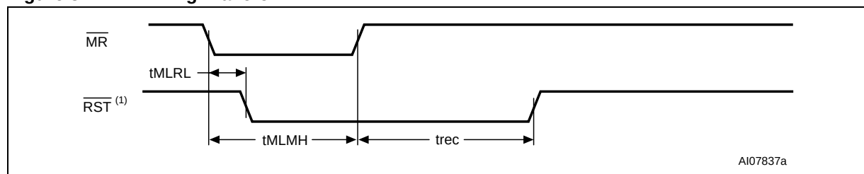
Figure 37. \overline{\text{MR}} Timing Waveform
