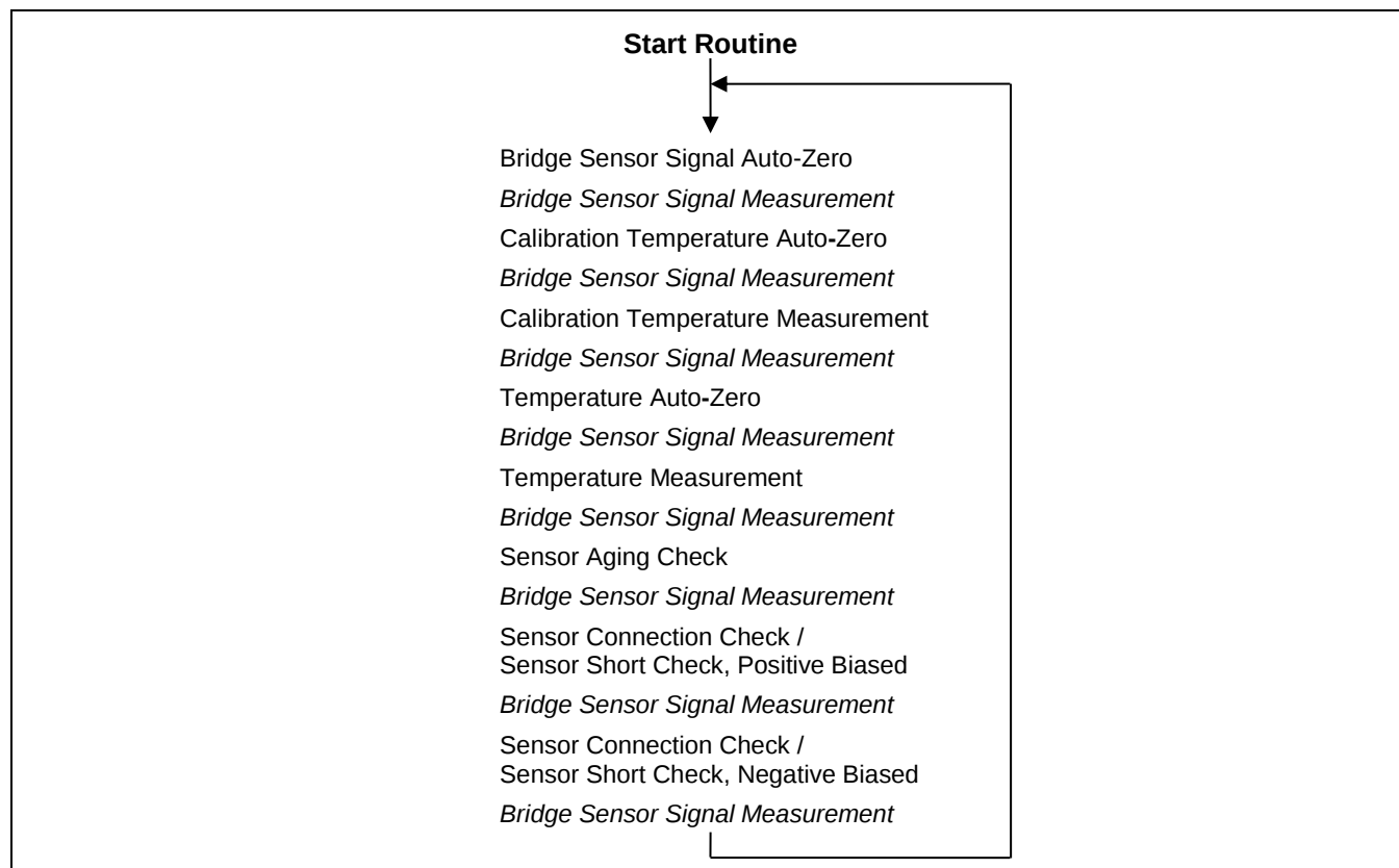
Figure 2.2 Measurement Cycle
