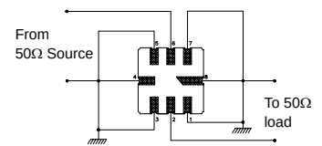
Test Circuit
