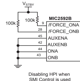
Figure 6. Input Pin Configuration for Disabling HPI/SMI Control
