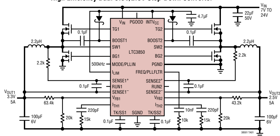
High Efficiency Dual 3.3V/2.5V Step-Down Converter
