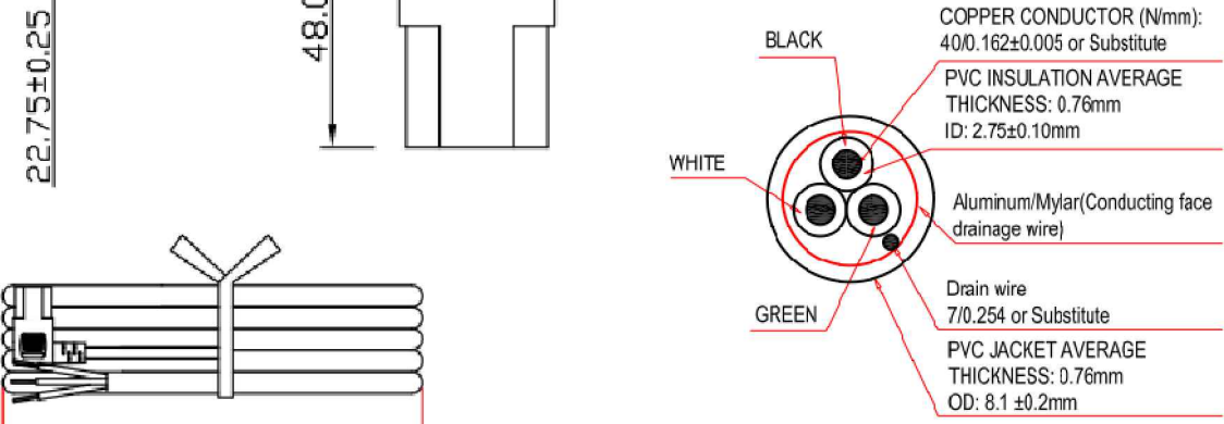
Wire cross section
