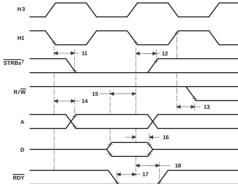
Figure 16. Memory-Read-Cycle Timing
