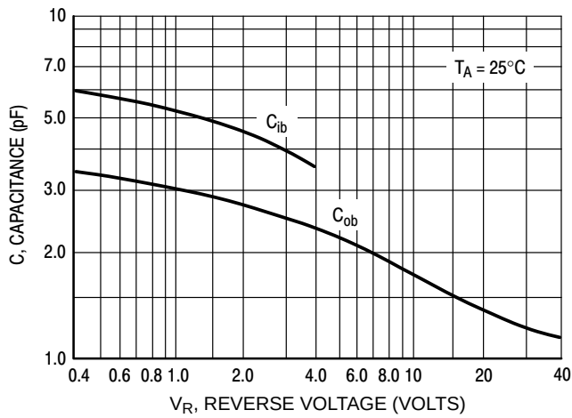
Figure 8. Capacitances
