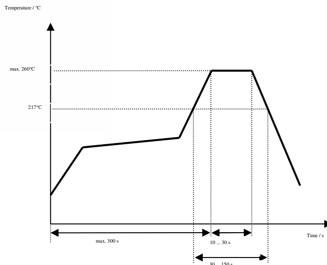
Chip-mount air reflow profile
