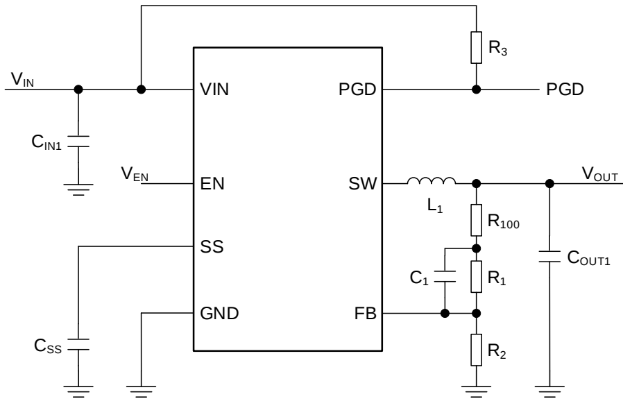
Figure 29. Reference Circuit 1
