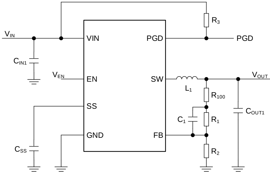
Figure 34. Reference Circuit 2
