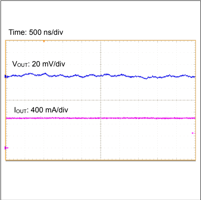
Figure 43. Output Ripple Voltage ( I_{OUT} = 1\text{ A} )
