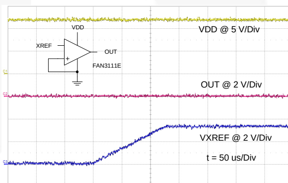
Figure 37. FAN3111E Startup Operation
