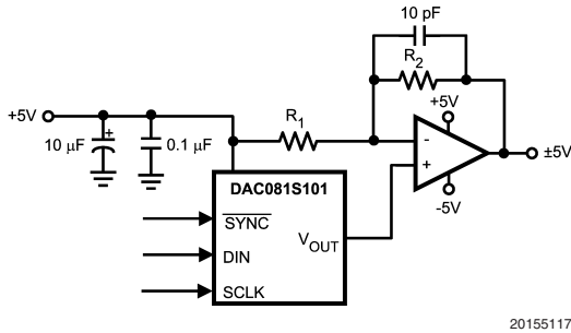
FIGURE 13. Bipolar Operation
