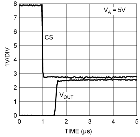
5V Wake-Up Time
