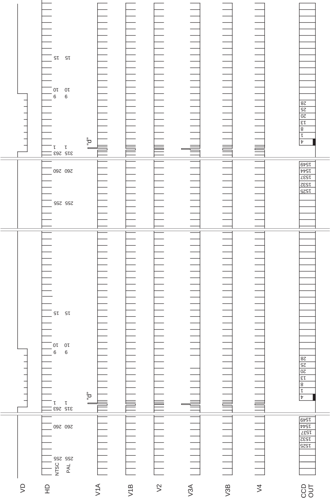
Drive Timing Chart (Vertical Sync) NTSC/PAL High Frame Rate Readout Mode NTSC: 30 frame/s, PAL: 25 frame/s
