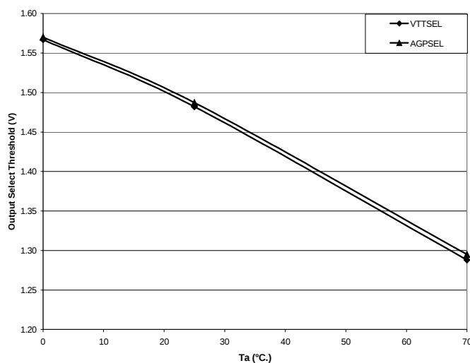
Output Select Threshold vs Ta
