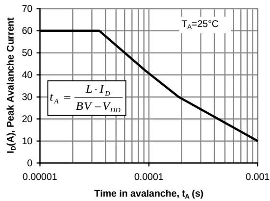
Figure 12: Avalanche capability
