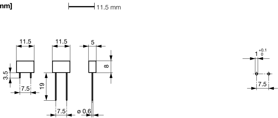
Drilling diagram
