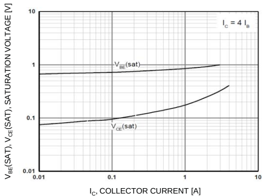
Figure 2. Base-Emitter Saturation Voltage Collector-Emitter Saturation Voltage
