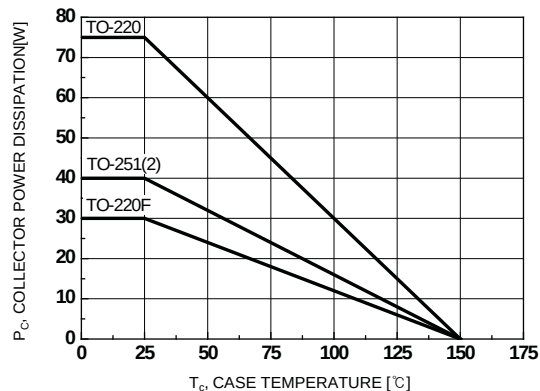
Figure 8. Power Derating
