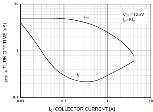
Figure 5. Turn Off Time
