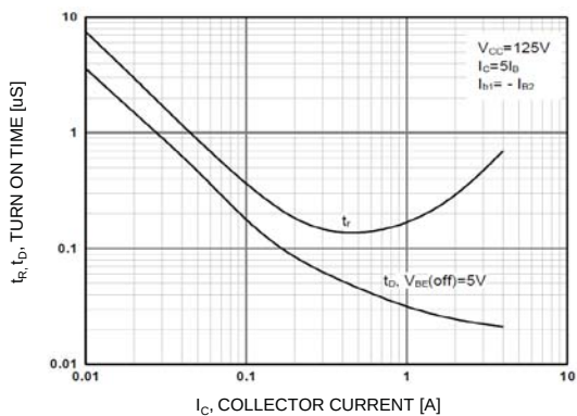
Figure 4. Turn On Time
