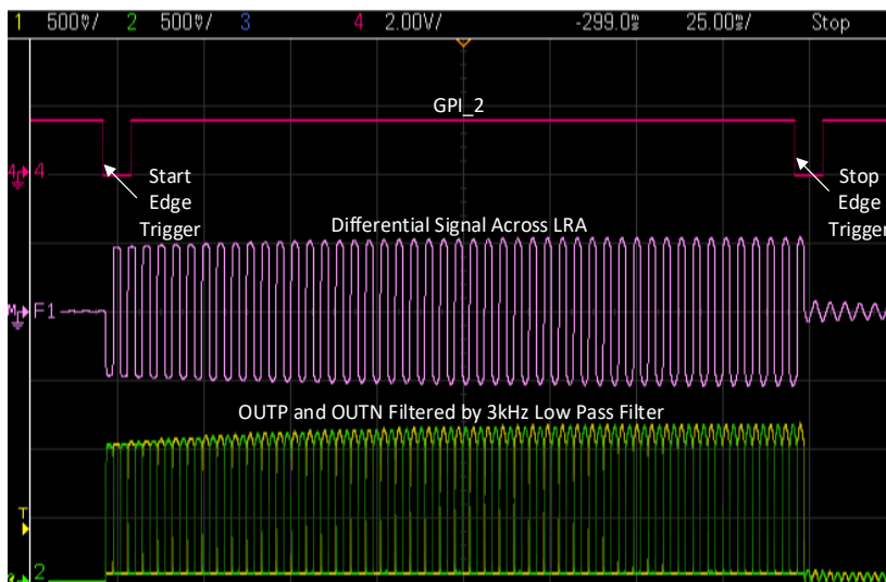
Figure 9: 200 ms Haptic Sequence Oscilloscope Image
