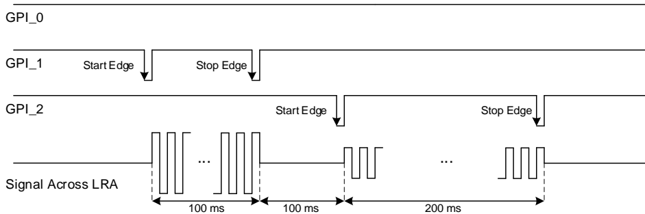
Figure 8: Complex Sequence Generation using GPIs
