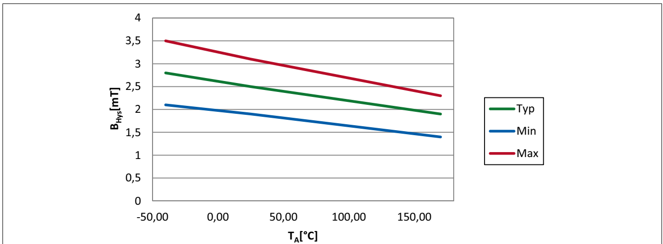
Figure 5-3 Hysteresis (B Hys ) of the TLE4964-5M over Temperature
