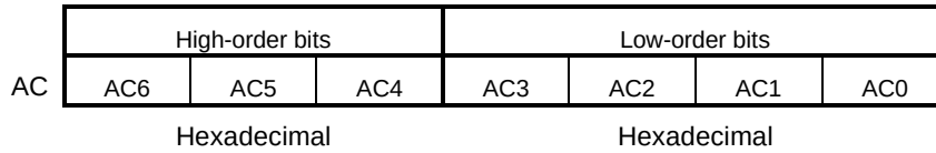
Figure 7–1. DDRAM Address
