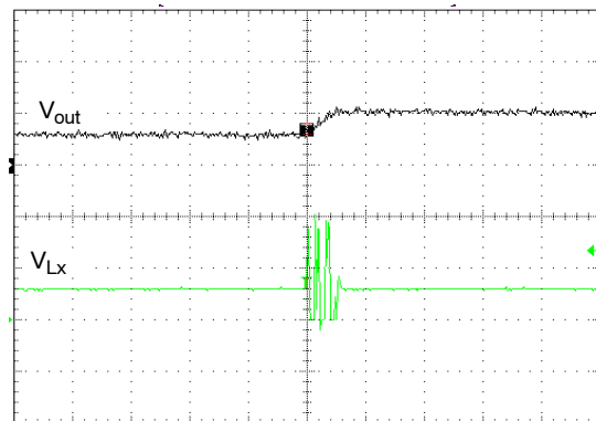
Figure 28. PFM Switching Waveforms ( V_{IN} = 3.6\text{ V} , V_{OUT} = 1.2\text{ V} , I_{OUT} = 0\text{ mA} , Temp = 25°C)
