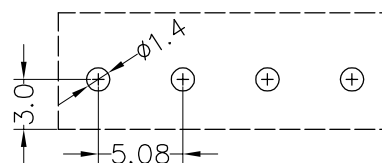
Recommended P.C.B Layout(Top Side)
