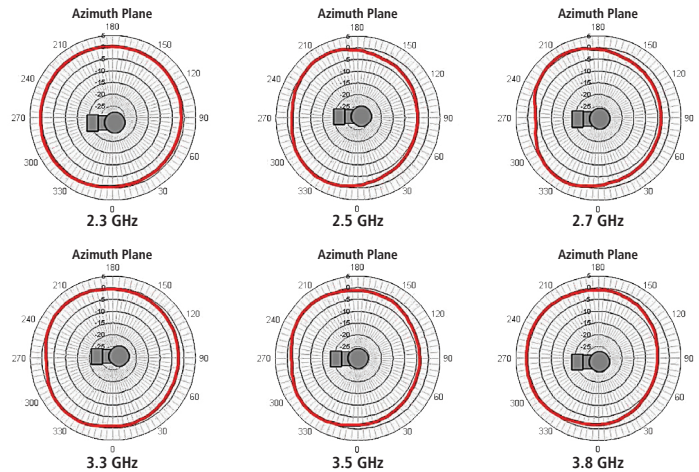
Typical Radiation Patterns (Azimuth Plane - Theta 90°)
