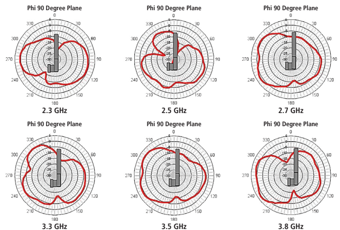
Typical Radiation Patterns (Elevation 90° Plane - Phi 90°)
