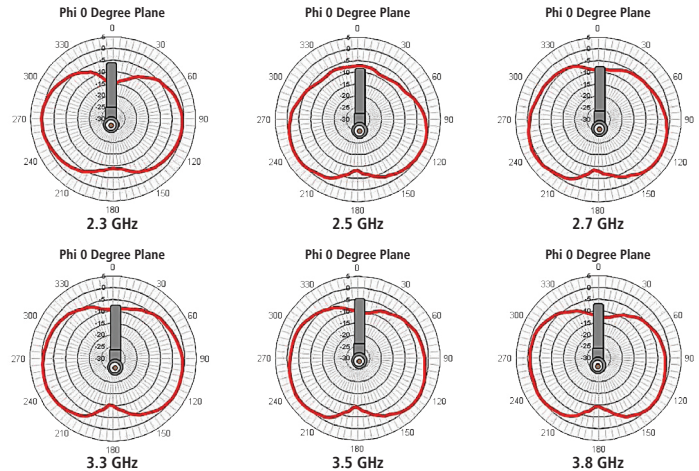
Typical Radiation Patterns (Elevation 0° Plane - Phi 0°)
