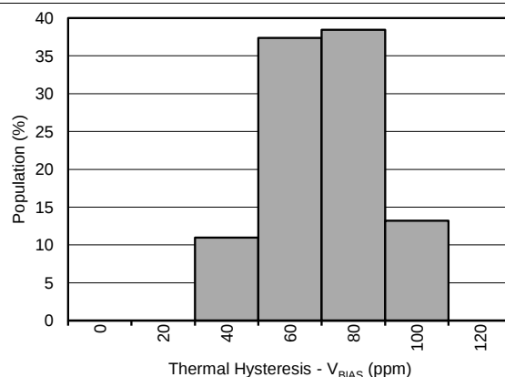
Figure 44. Thermal Hysteresis Distribution (V BIAS )
