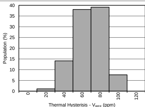
Figure 43. Thermal Hysteresis Distribution (V REF )
