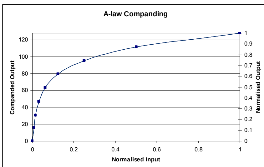
Figure 51 A-Law Companding
