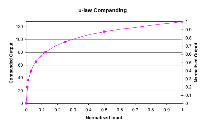
Figure 50 \mu -Law Companding
