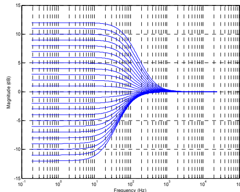
Figure 65 EQ Band 1 Gains for Lowest Cut-off Frequency
