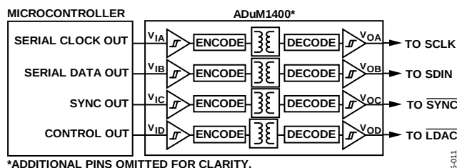
Figure 51. Isolated Interface
