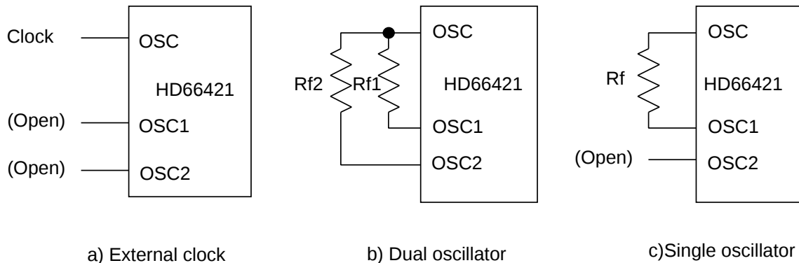
Figure 30 Oscillator Connections
