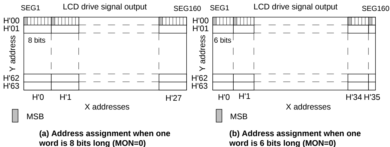
Figure 11 Display RAM Addresses in Gray Scale Mode
