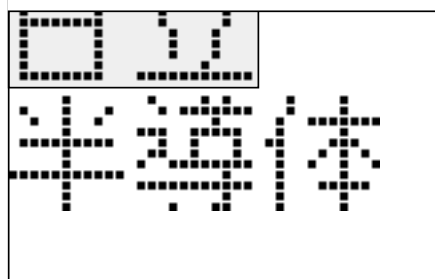
Figure 25 Blink Area Designation by Blink Control Registers
