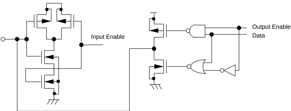
Figure 47 Terminal Configuration
