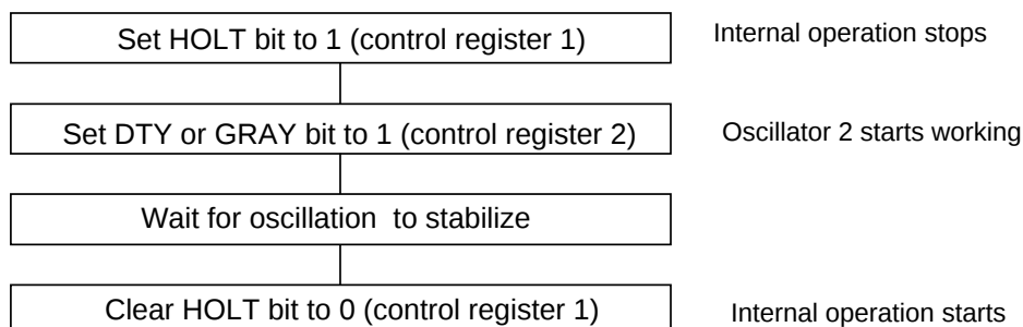
Figure 28 Procedure for Changing Oscillator
