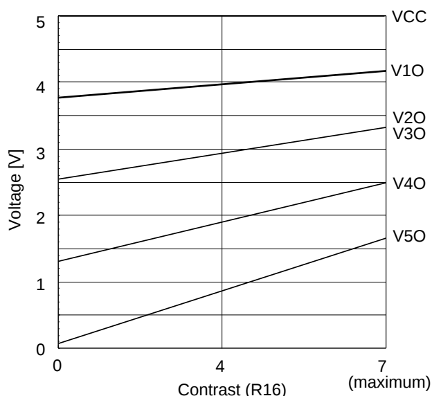
Example 2. LCD bias level
