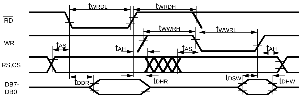
Figure 44 MPU Interface
