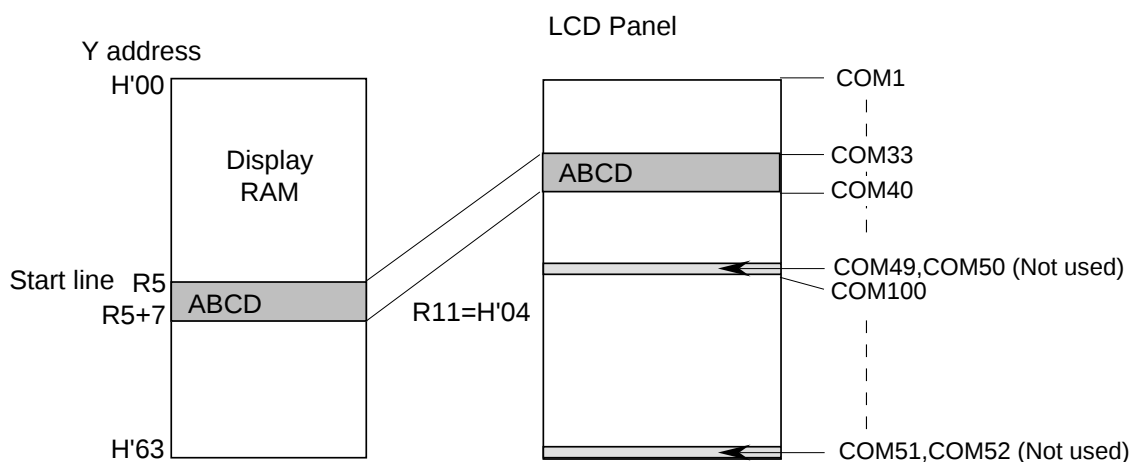
Figure 24 Partial Display
