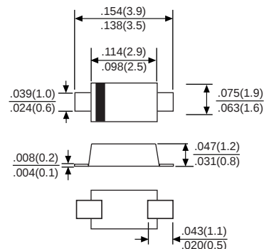
SOD-123FL
