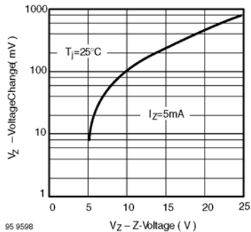
Fig. 2 Typical Change of Working Voltage under Operating Conditions at T_{\text{amb}}=25^{\circ}\text{C}
