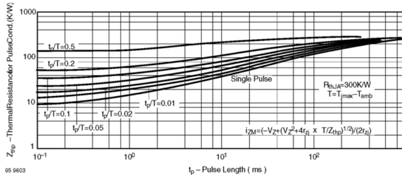
Fig. 10 Thermal Response
