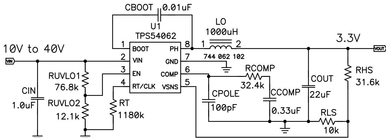
Figure 36. DCM 应用原理图
