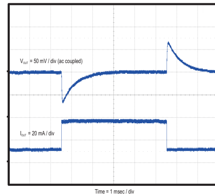
Figure 26. 负载瞬态
