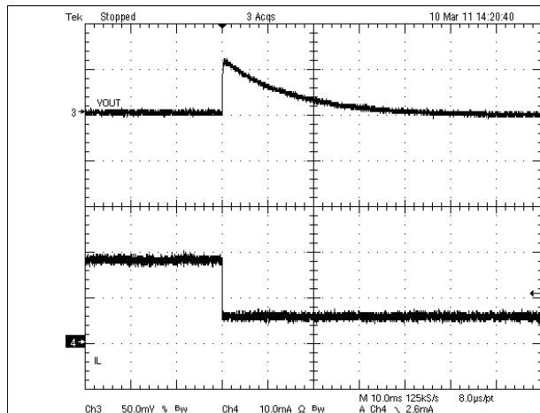
Figure 43. 空载瞬态
