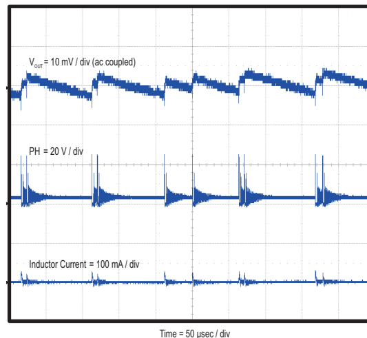
Figure 35. 输出纹波跳跃
