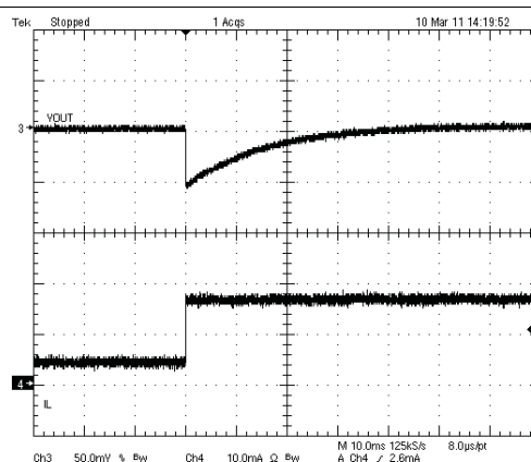
Figure 42. 负载瞬态
