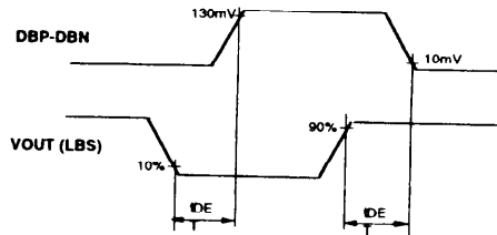
DETECTOR PROPAGATION DELAY
