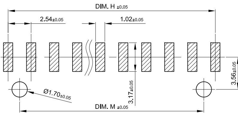
PCB Layout
