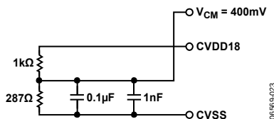
Figure 31. DAC Clock VCM Circuit
