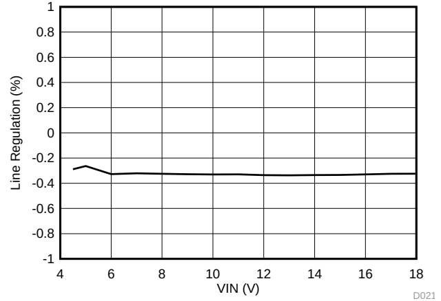
Figure 25. Line Regulation, I_{OUT} = 6\text{ A}
