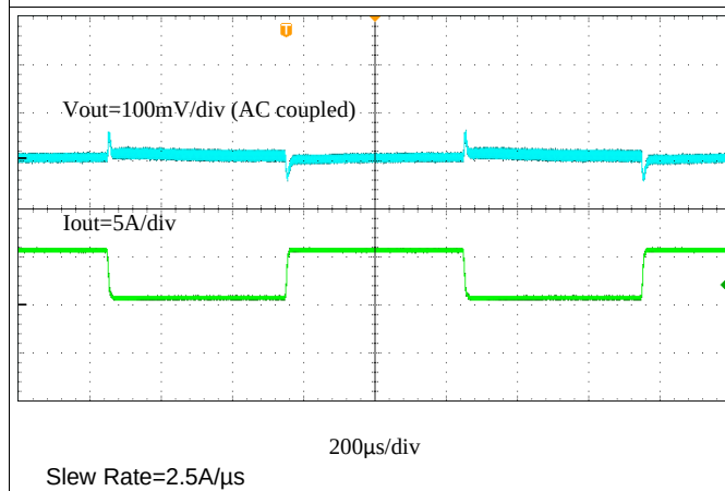
Figure 32. Transient Response, 0.6 A to 5.4 A
