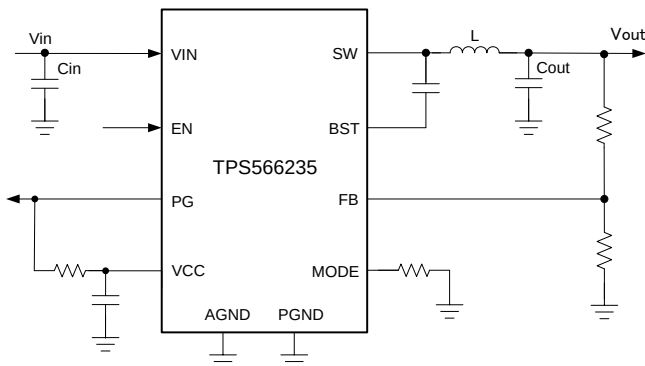
Typical Application
