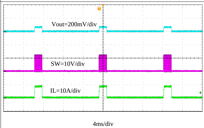
Figure 35. Output Hard Short Hiccup
