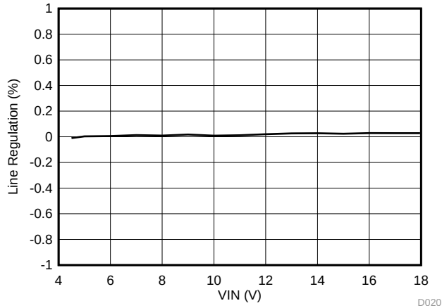
Figure 24. Line Regulation, I_{OUT} = 0.01\text{ A}
