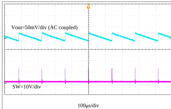
Figure 30. Output Voltage Ripple, I_{OUT} = 0.01 A
