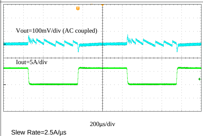
Figure 33. Transient Response, 0 A to 6 A
