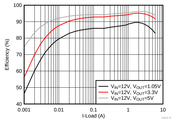
Efficiency vs Output Current Eco-mode
