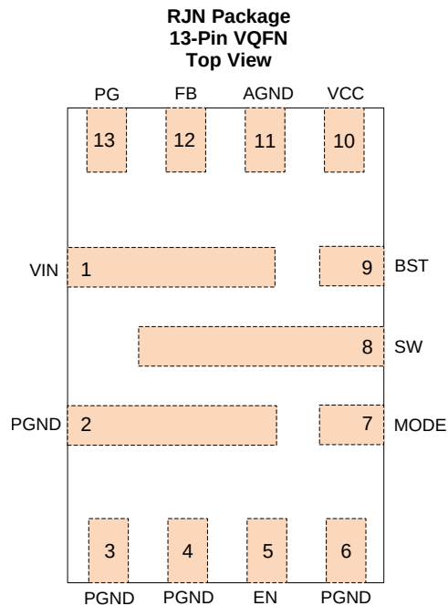
Pin Functions
