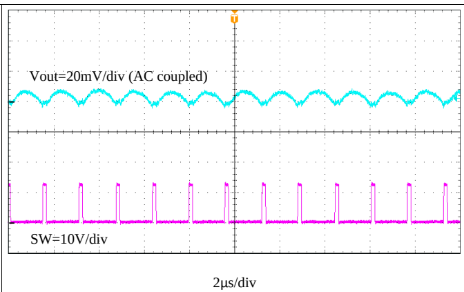
Figure 31. Output Voltage Ripple, I_{OUT} = 6 A
