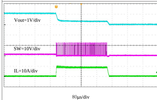
Figure 32. Transient Response, 0.6 A to 5.4 A
