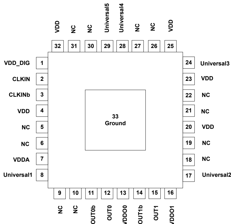
Figure 6.8. Si53352A-Dxxxxx-AM 32-QFN
