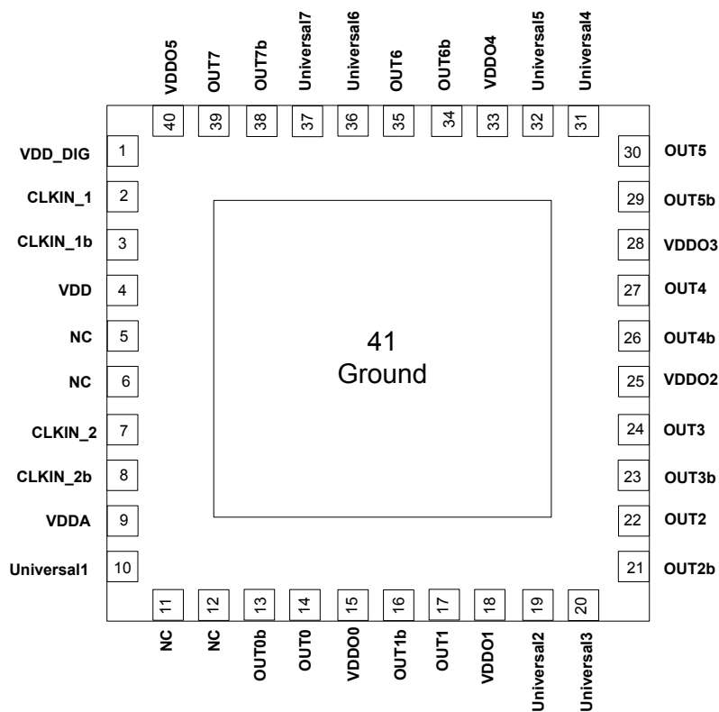
Figure 6.4. Si53358Bxxxxx-AM 40-QFN
