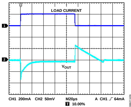
图28. 输出瞬态响应( C_{OUT} = 1 \mu\text{F} )
