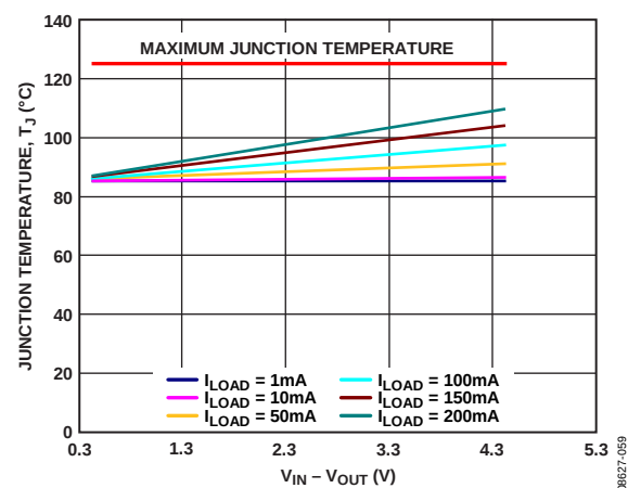
图59. LFCSP封装, T_A = 85^\circ\text{C}
