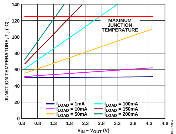
图56. LFCSP 50 mm² PCB覆铜, T_A = 50^\circ C
