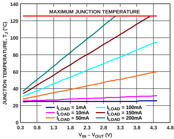
图41. WLCSP 50 mm 2 PCB覆铜, T_A = 25^{\circ}\text{C}
