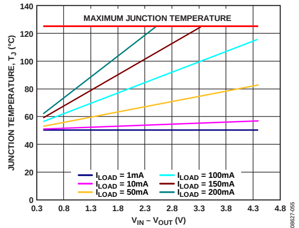
图54. LFCSP 500 mm² PCB覆铜, T_A = 50^\circ C
