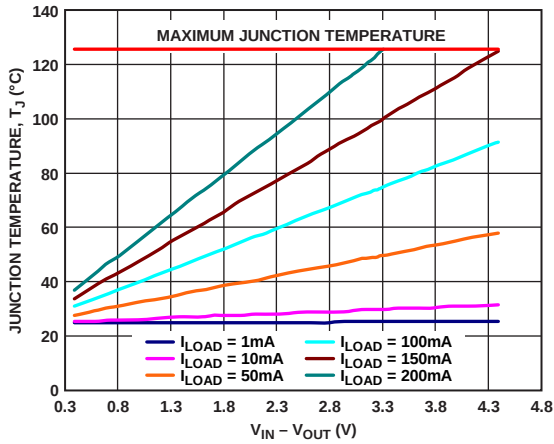
图39. WLCSP 500 mm 2 PCB覆铜, T_A = 25^{\circ}\text{C}
