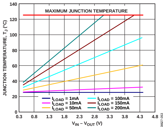
图53. LFCSP 50 mm² PCB覆铜, T_A = 25^\circ C
