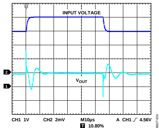
图26. 线路瞬态响应 ( C_{IN} , C_{OUT} = 1 \mu F , I_{LOAD} = 1 \text{ mA} )
