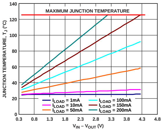
图40. WLCSP 100 mm 2 PCB覆铜, T_A = 25^{\circ}\text{C}
