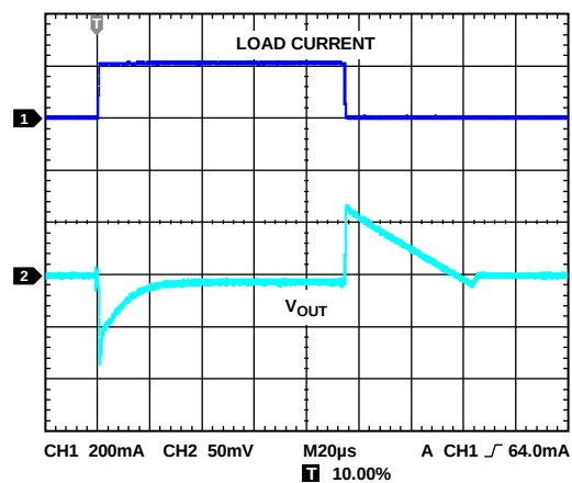
图24. 负载瞬态响应 ( C_{IN} , C_{OUT} = 1\text{ μF} , I_{LOAD} = 1\text{ mA} 至 200\text{ mA} )
