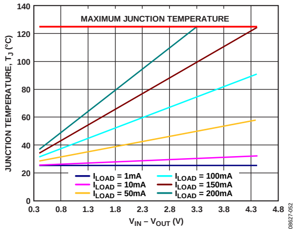
图52. LFCSP 100 mm² PCB覆铜, T_A = 25^\circ C
