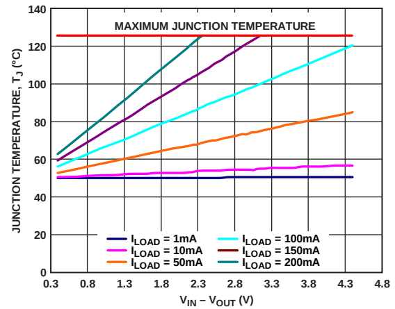
图44. WLCSP 50 mm 2 PCB覆铜, T_A = 50^{\circ}\text{C}
