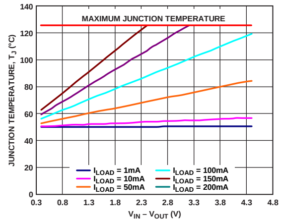
图43. WLCSP 100 mm 2 PCB覆铜, T_A = 50^{\circ}\text{C}
