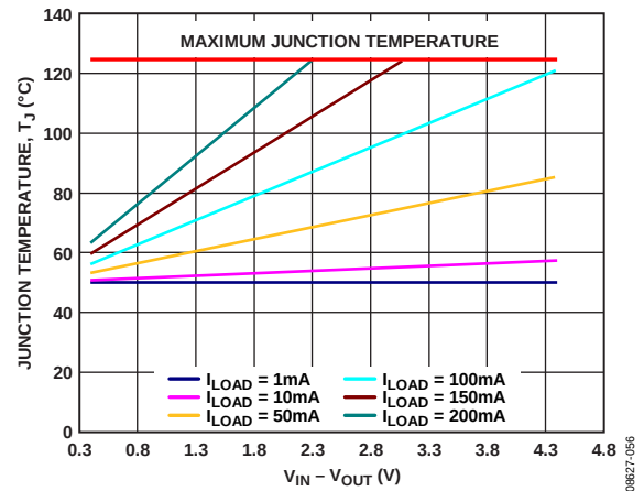
图55. LFCSP 100 mm² PCB覆铜, T_A = 50^\circ C
