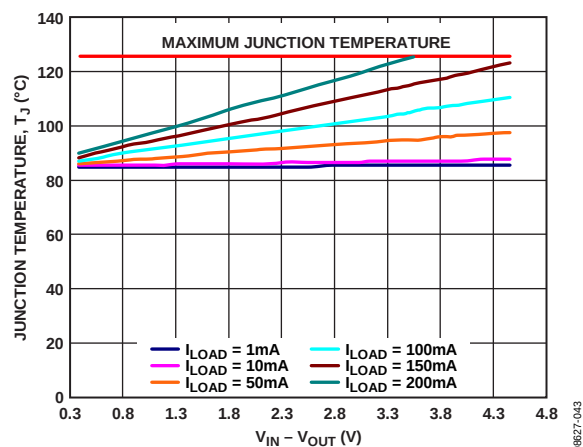
图57. WLCSP封装, T_A = 85^\circ\text{C}
