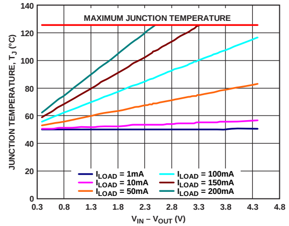
图42. WLCSP 500 mm 2 PCB覆铜, T_A = 50^{\circ}\text{C}
