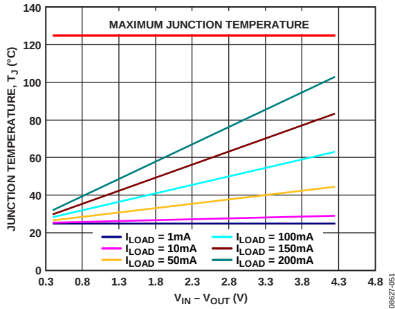
图51. LFCSP 500 mm² PCB覆铜, T_A = 25^\circ C
