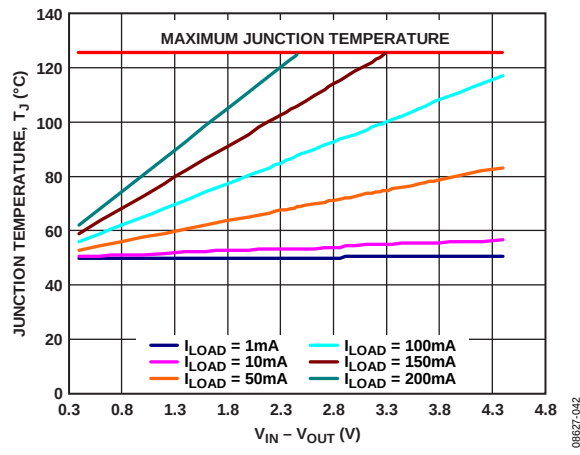
图50. TSOT 50 mm² PCB覆铜, T_A = 50^\circ C
