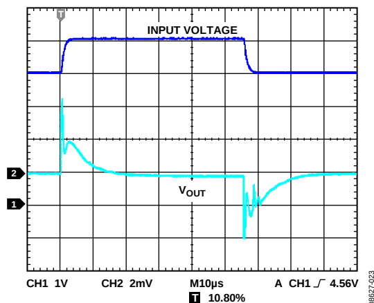
图25. 线路瞬态响应 ( C_{IN} , C_{OUT} = 1 \mu F , I_{LOAD} = 200 \text{ mA} )
