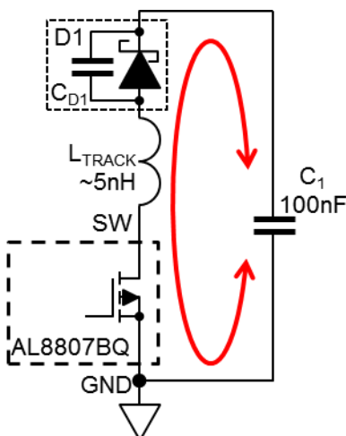
Figure 41 PCB Loop Resonance
