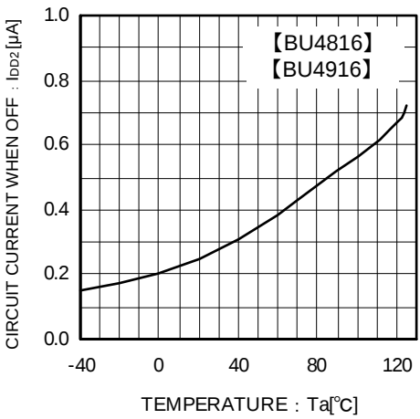
Fig.10 Circuit Current when OFF
