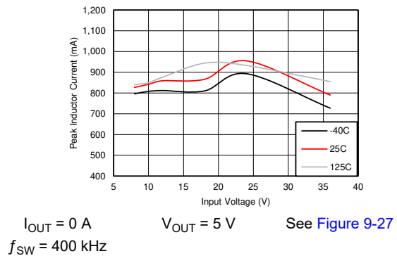
Figure 7-6. I_{PEAK-MIN}
