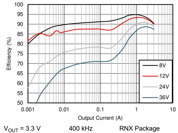
Figure 9-6. Efficiency
