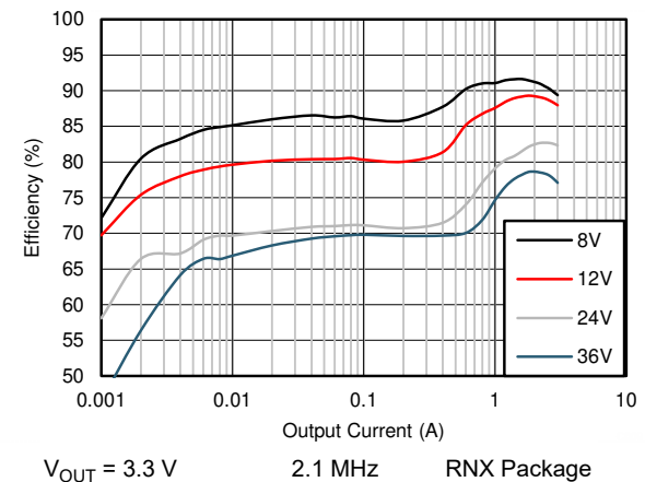
Figure 9-8. Efficiency
