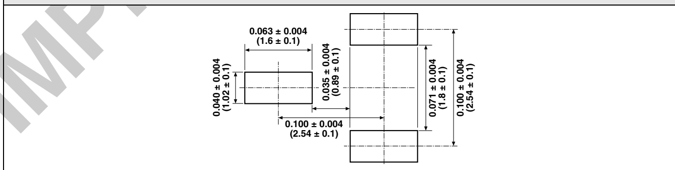
FIGURE 6 - RECOMMENDED LAND PATTERN
