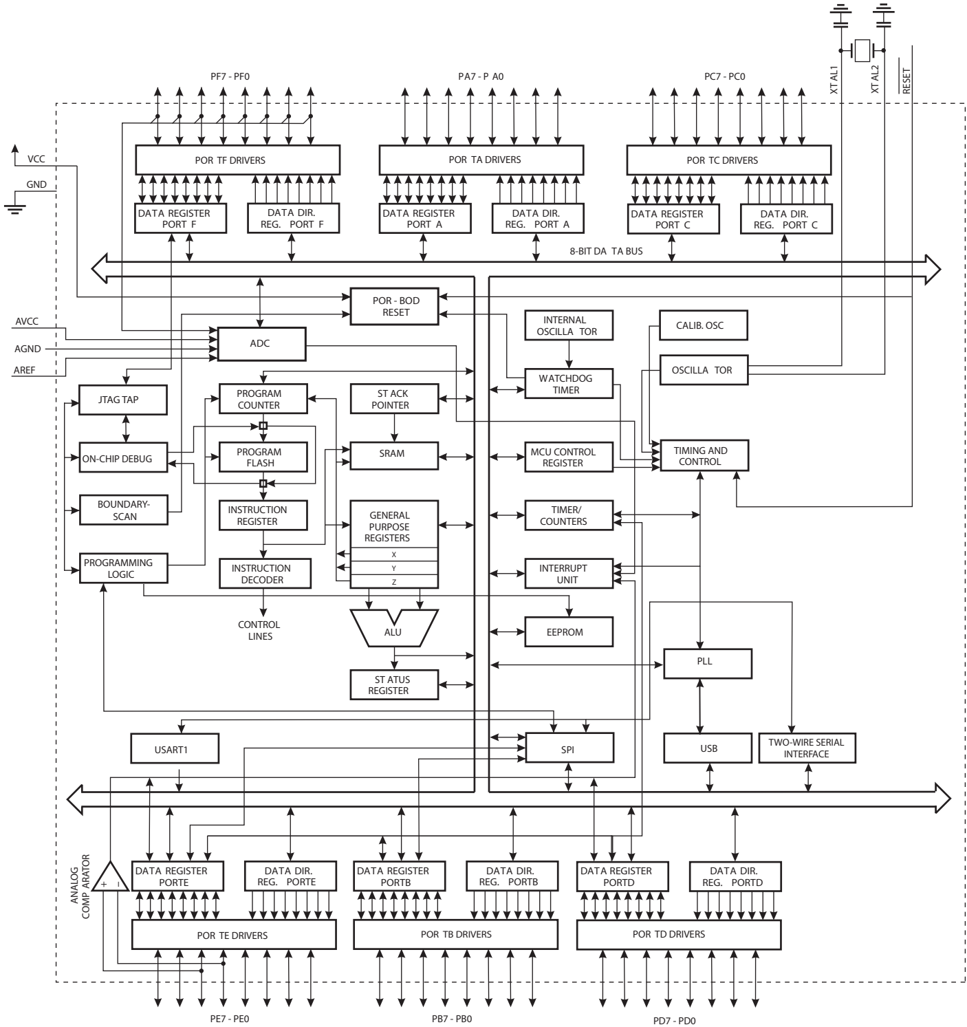
Figure 2-1. Block diagram.
