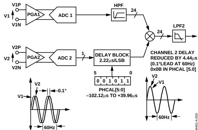
Figure 49. Phase Calibration
