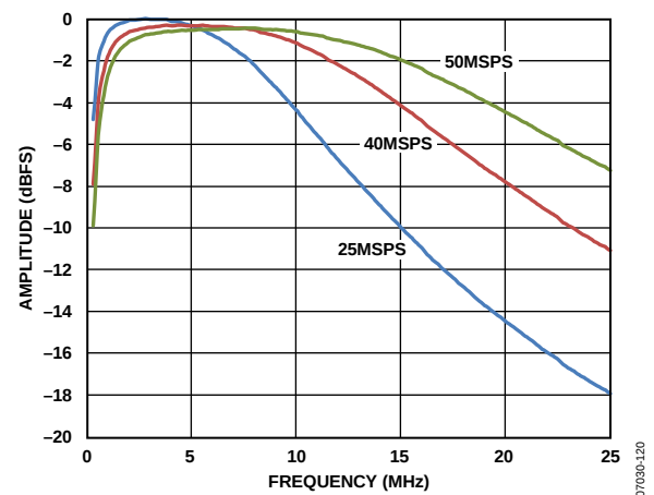
图17.抗混叠滤波器(AAF)通带响应, LPF 截止频率 = 1 \times (1/3) \times f_{SAMPLE}
