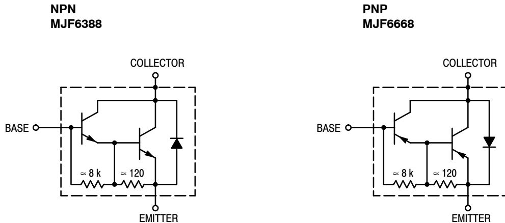
Figure 1. Darlington Schematic
