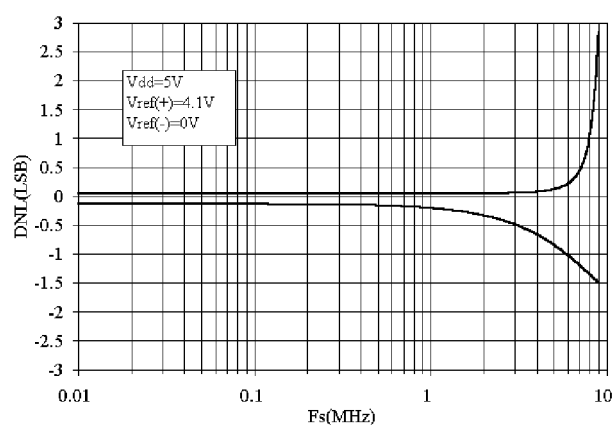
Graph 6. DNL vs. Sampling Frequency
