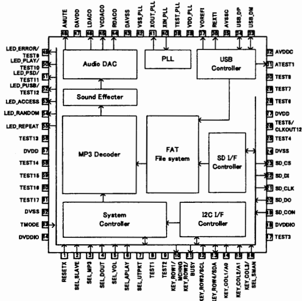
Figure 2. Block diagram
