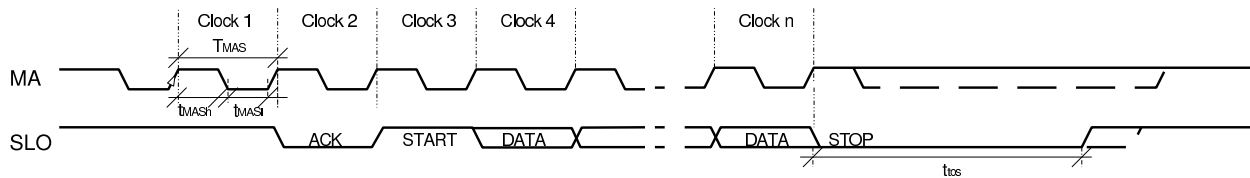
Figure 4: Timing diagram in BiSS C protocol.
